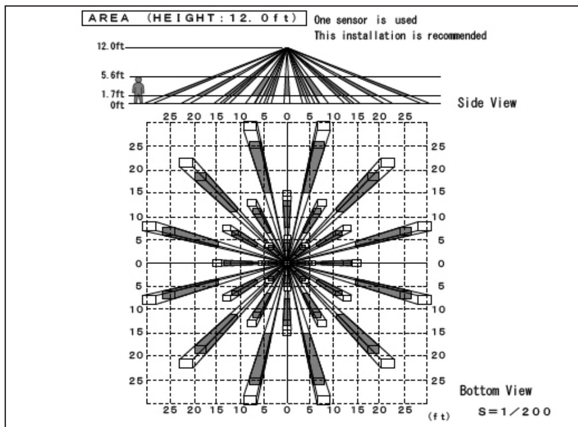
Figure 8: 1126 12' Detection Pattern
