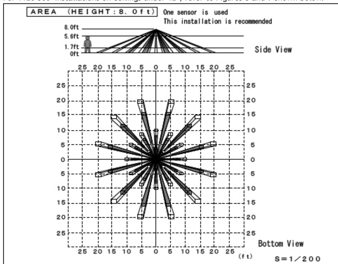
Figure 7: 1126 8' Detection Pattern
