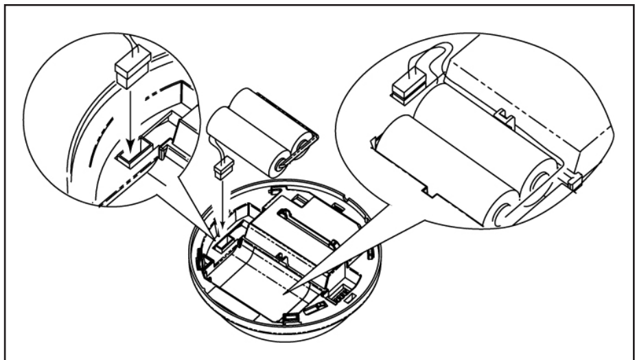
Figure 11: Battery Replacement
